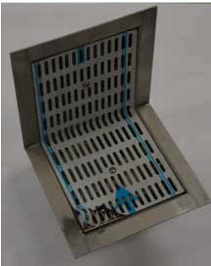
Customised ACO Parapet outlet with slotted screwed grating in stainless steel.
